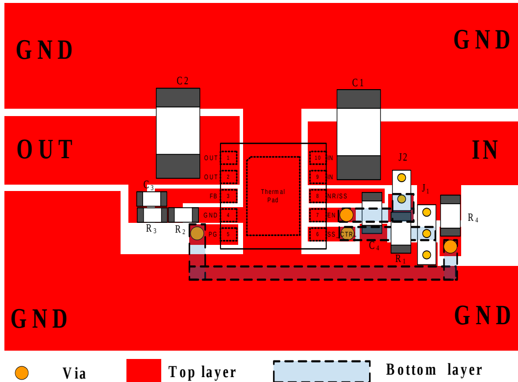
Figure3. PCB Layout Suggestion
