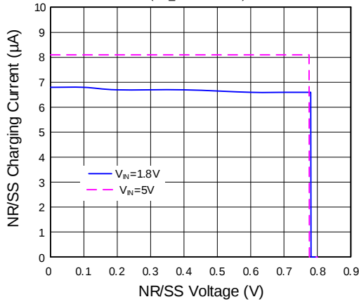
NR/SS Charging Current vs. NR/SS Voltage (SS_CTRL = GND)
