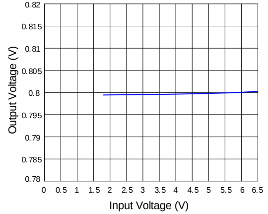
Line Regulation (I OUT =5mA)
