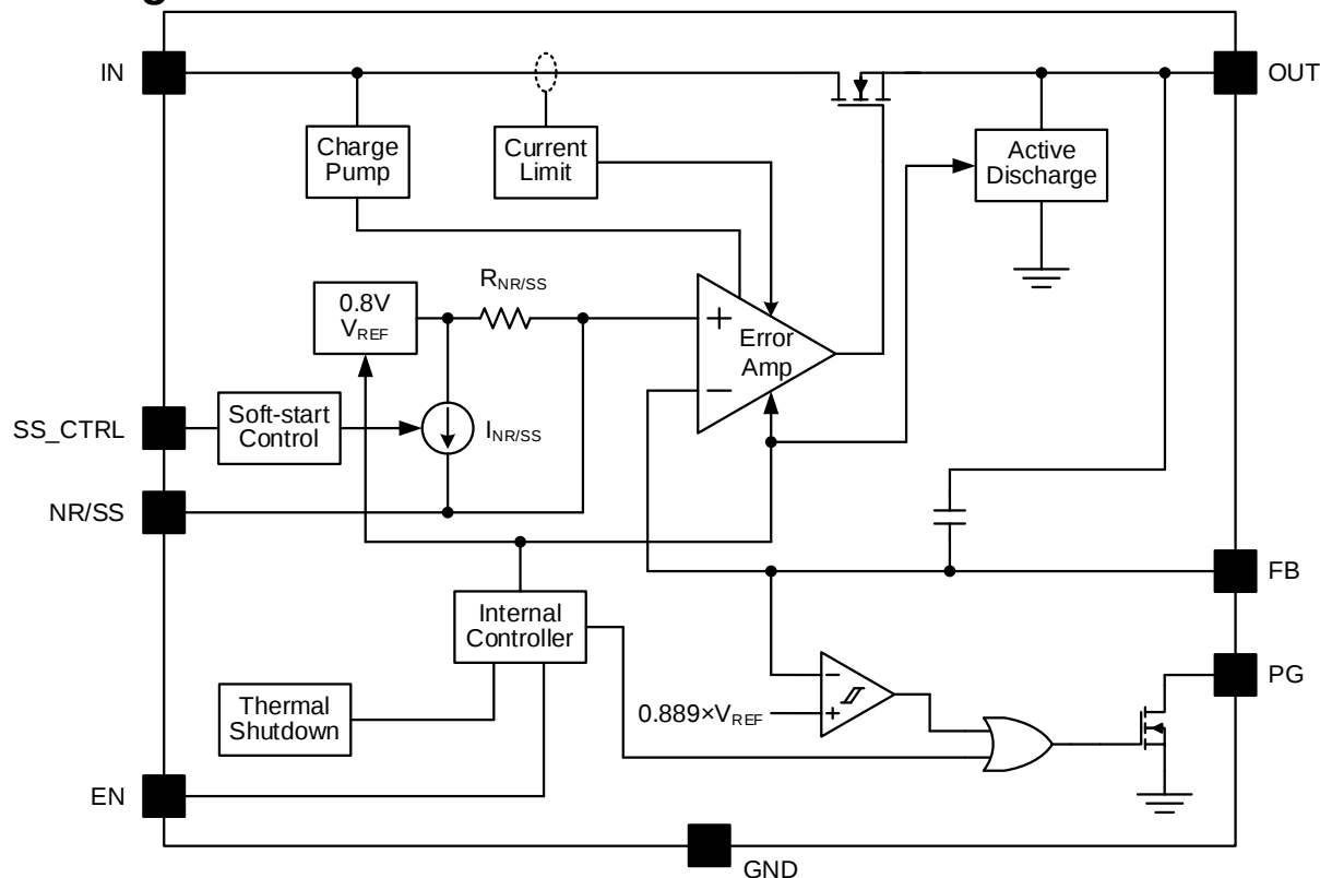
Figure2. Block Diagram
