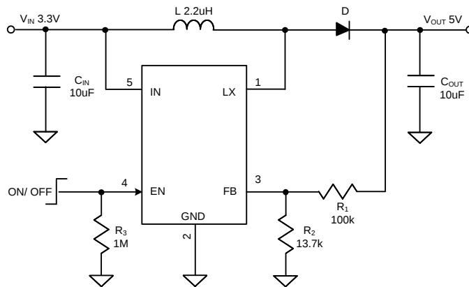
Figure 1. Schematic Diagram
