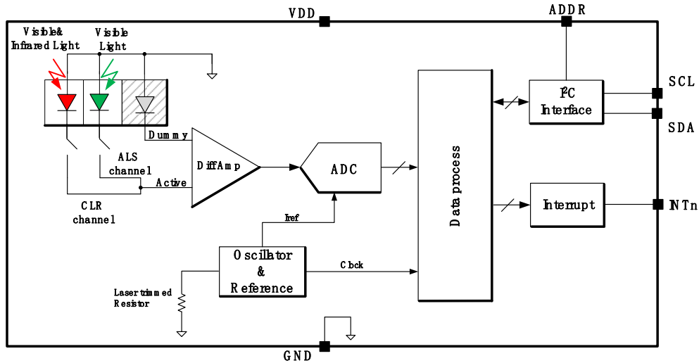
Figure 2. Block Diagram
